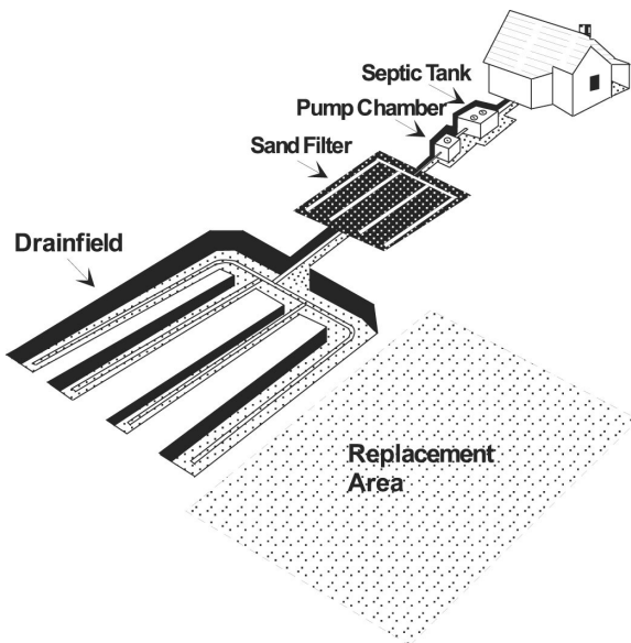
Image: Diagram of a basic septic system.
