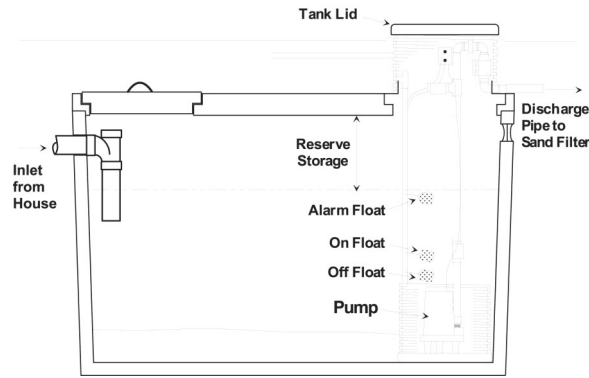
Image: Diagram of a pump tank.
